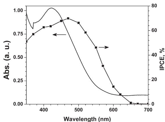
Fig. 3 Absorption spectrum of the dye 9 adsorbed on nanocrystalline TiO 2 and the action spectrum for the DSSC constructed using 9 .
